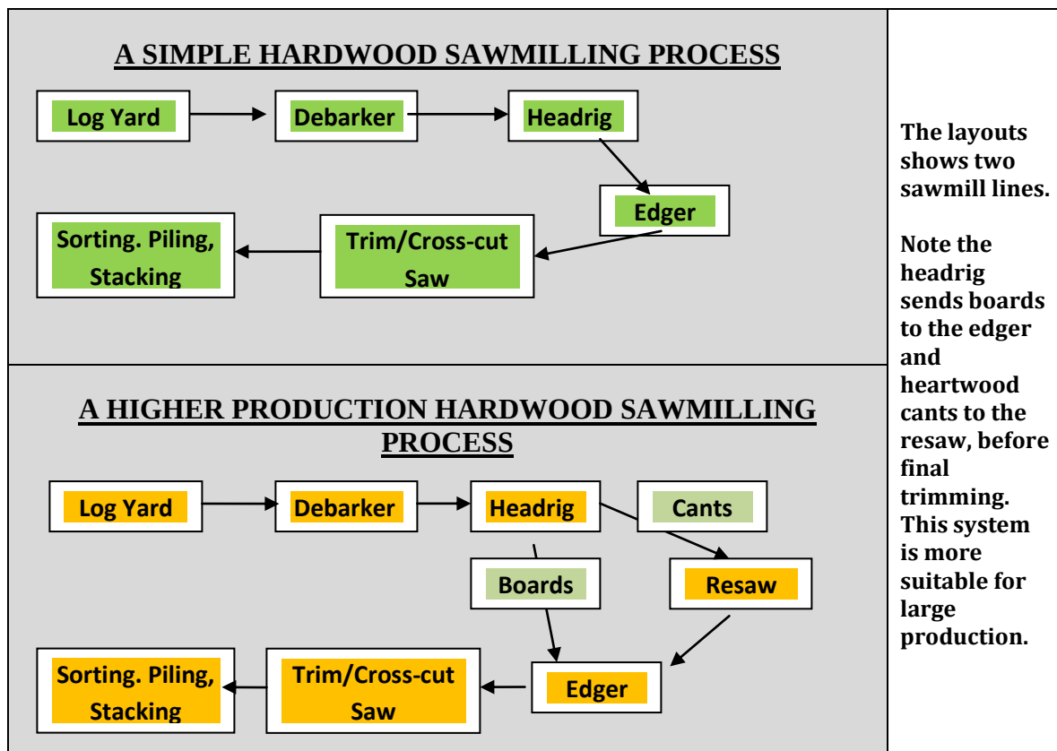
Figure 3: Simple sawmilling process flow
