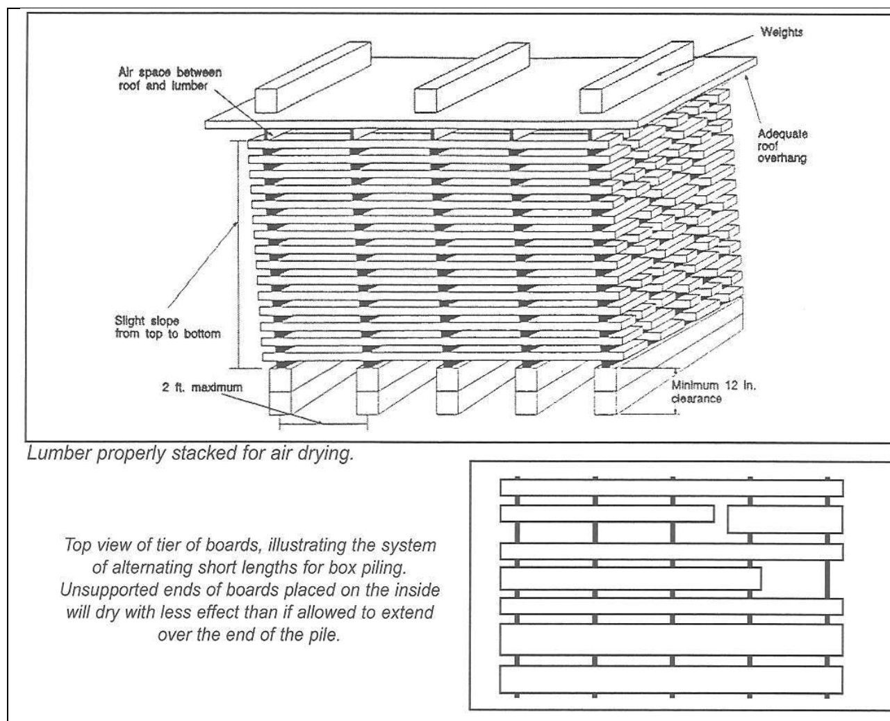
Figure 25: Stacking and Stickering of lumber
